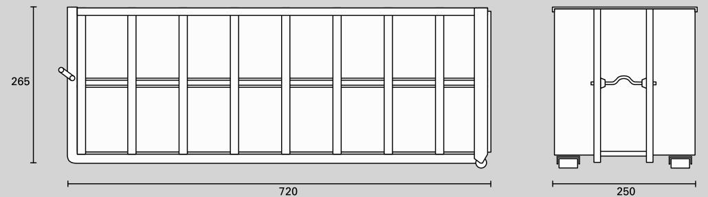
Abrollcontainer 40m 3
